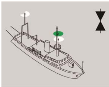
Vessel engaged in trawling—not making way; vessel over 50 meters in length.
